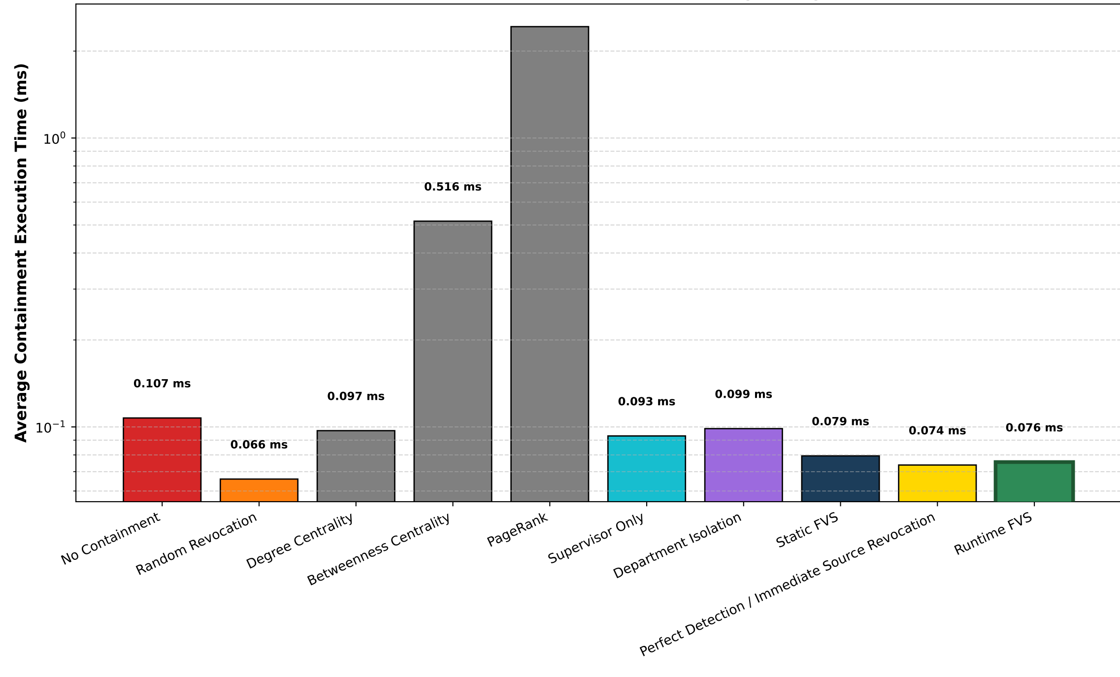
Computational Decision Overhead by Policy
